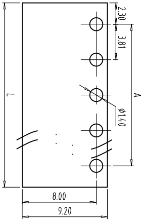
PCB LAYOUT S=3:1
