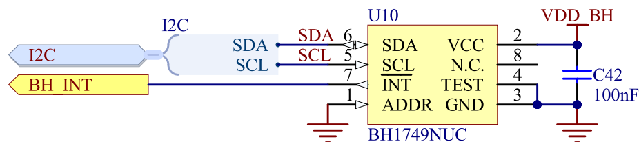
Figure 17: Color sensor
