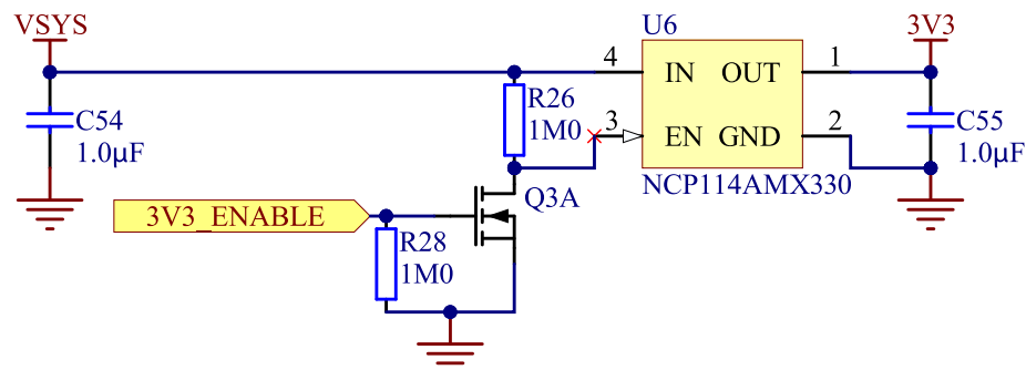
Figure 29: Regulator
