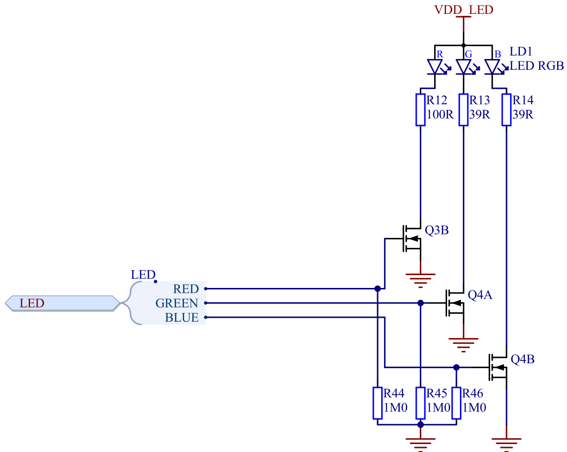
Figure 21: RGB LED
