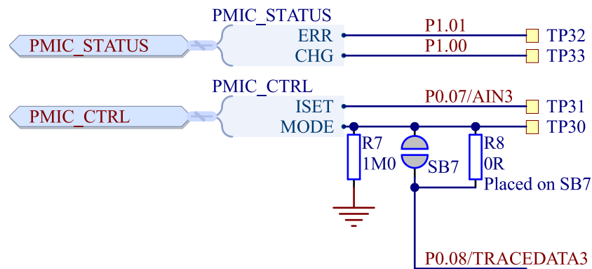
Figure 26: nPM1100 PMIC status and control on Thingy:53 v1.0.0
