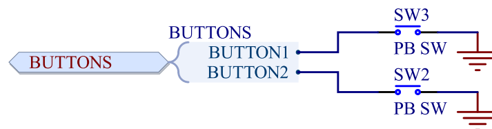
Figure 22: Buttons
