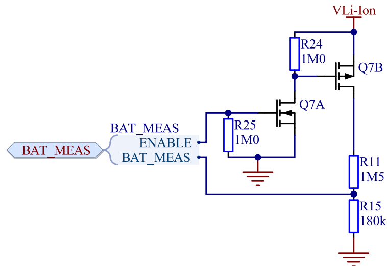
Figure 28: Battery voltage monitor
