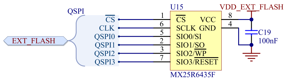
Figure 20: External memory
