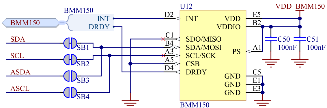
Figure 15: Magnetometer
