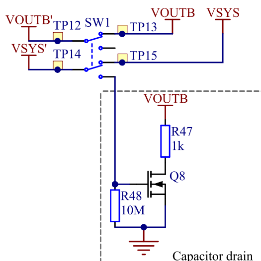
Figure 24: Power switch
