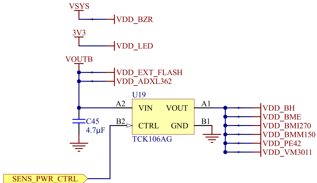
Figure 30: Sensor power control circuit
