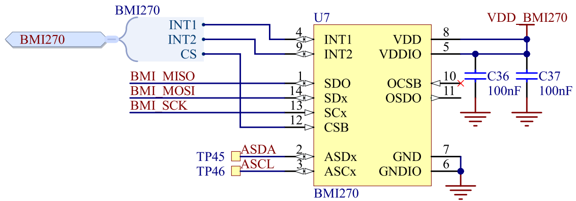
Figure 14: IMU
