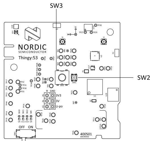
Figure 23: Nordic Thingy:53 buttons
