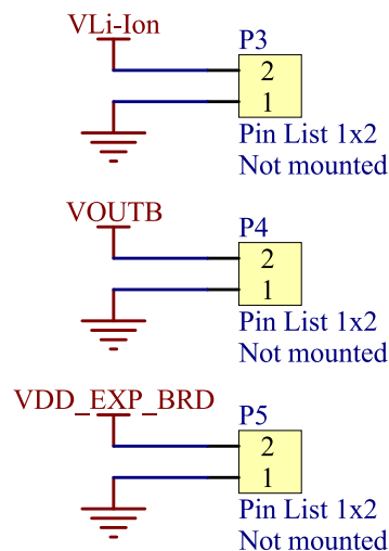
Figure 35: Power connectors
