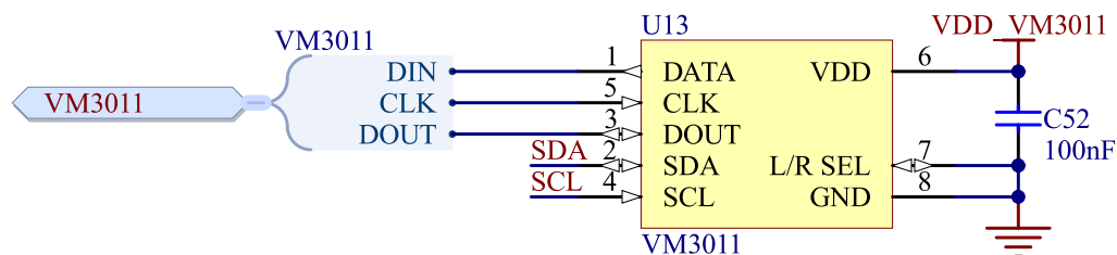
Figure 18: PDM microphone
