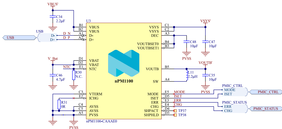
Figure 25: nPM1100 PMIC
