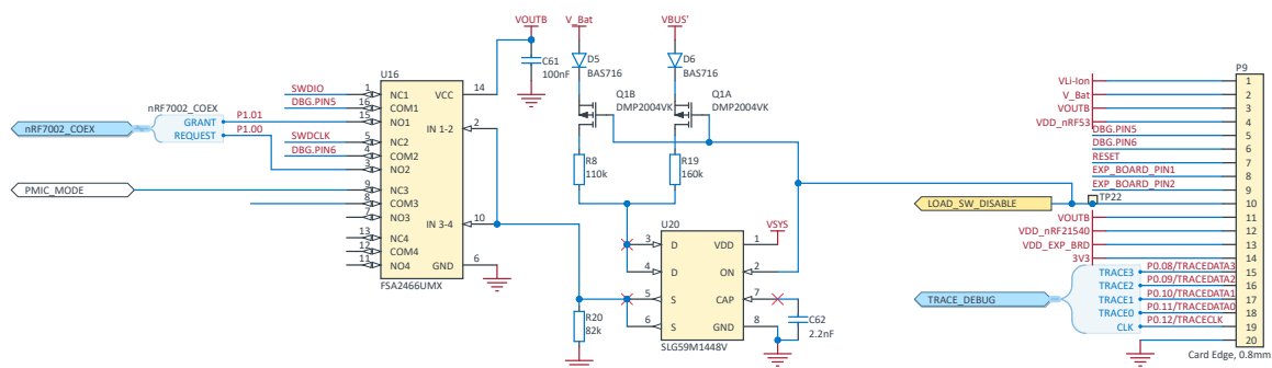
Figure 33: Signal switching circuit for nRF7002 EB
