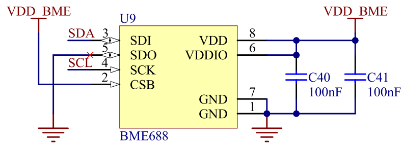
Figure 16: Environmental sensors
