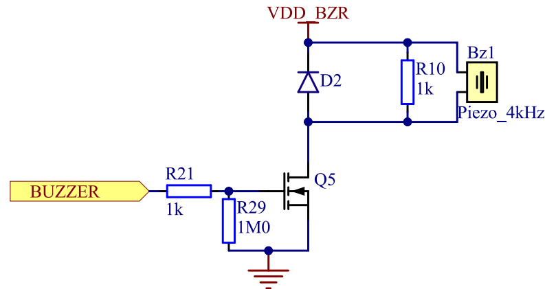
Figure 19: Buzzer
