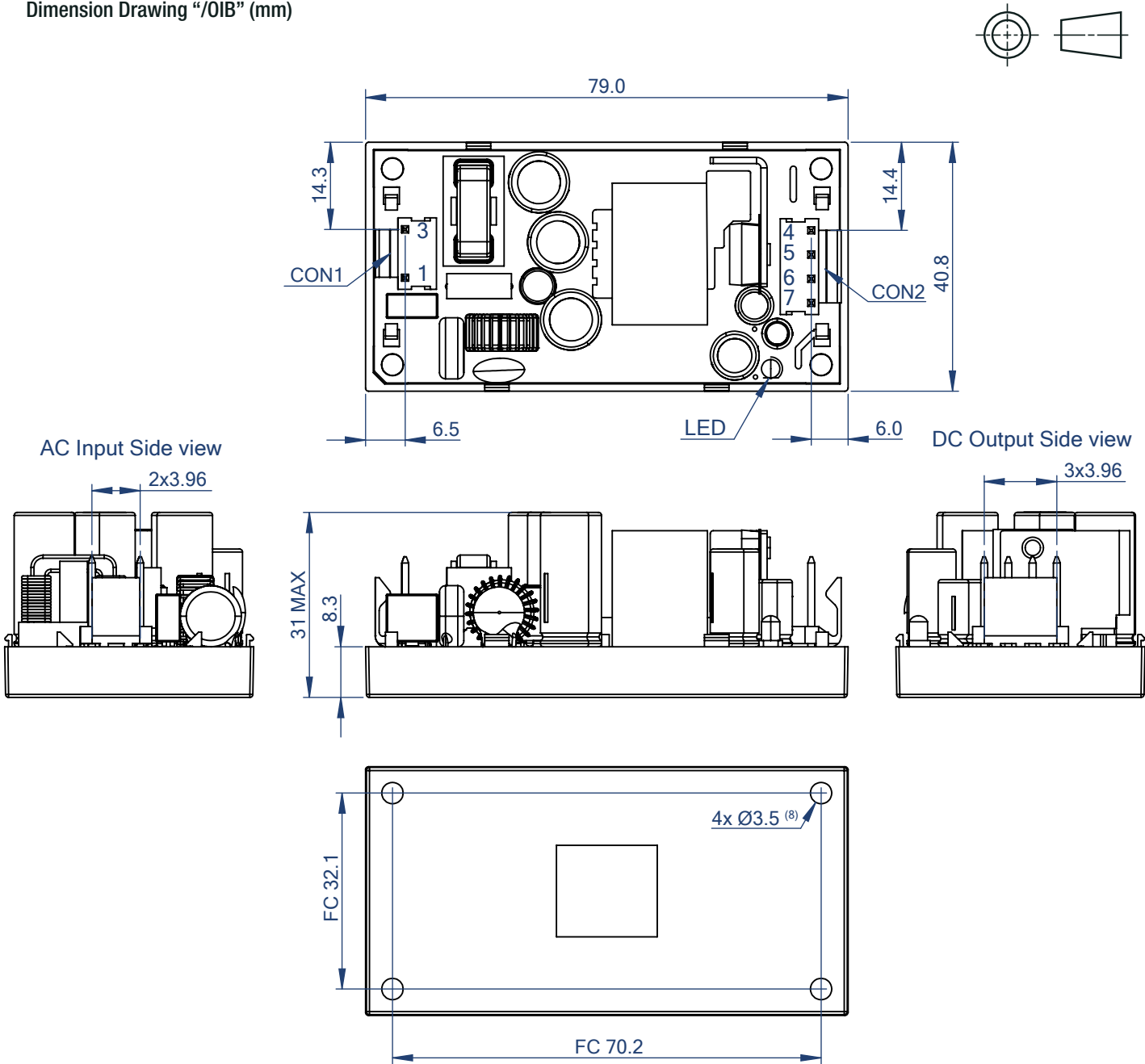
Dimension Drawing “/01B” (mm)
