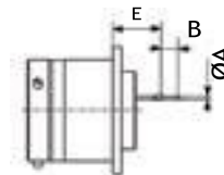
Type 2 Short square flange receptacle
