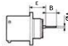
Type 3 Square flange receptacle (rear mounting)
