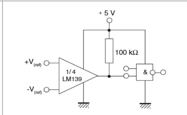
Figure 8. Driving CMOS
