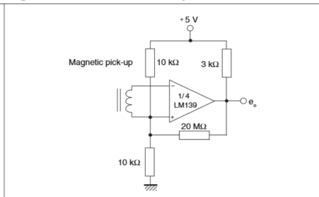
Figure 12. Transducer amplifier
