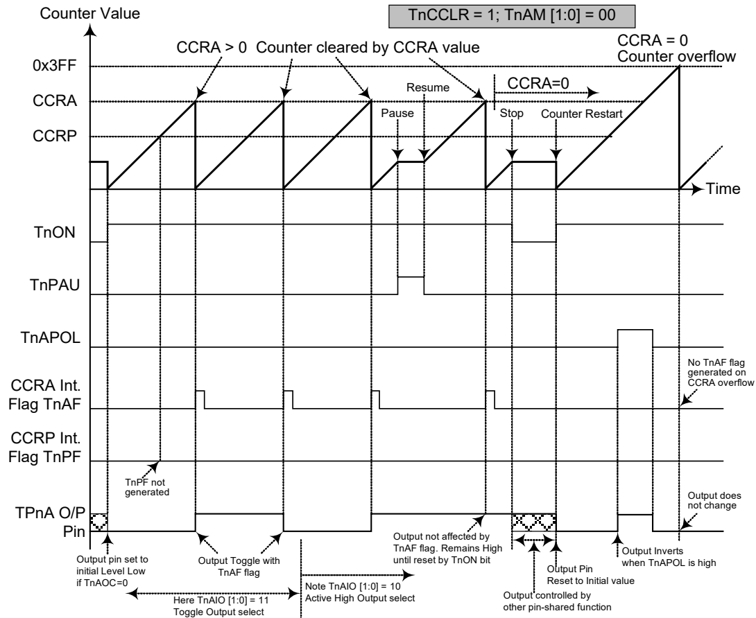
ETM CCRA Compare Match Output Mode – TnCCLR=1
