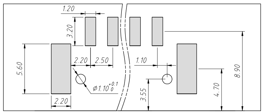
PCB Layout
