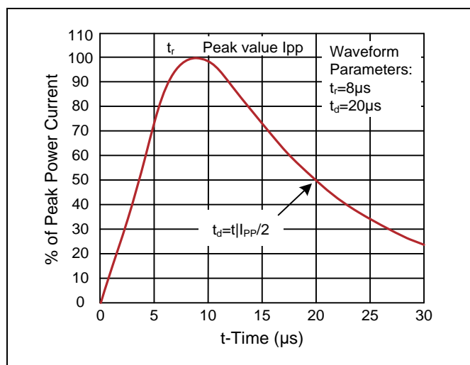
Figure 2. 8/20 \mu s Pulse Waveforms
