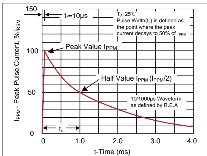
Figure 5. 10/1000μs Pulse Waveform
