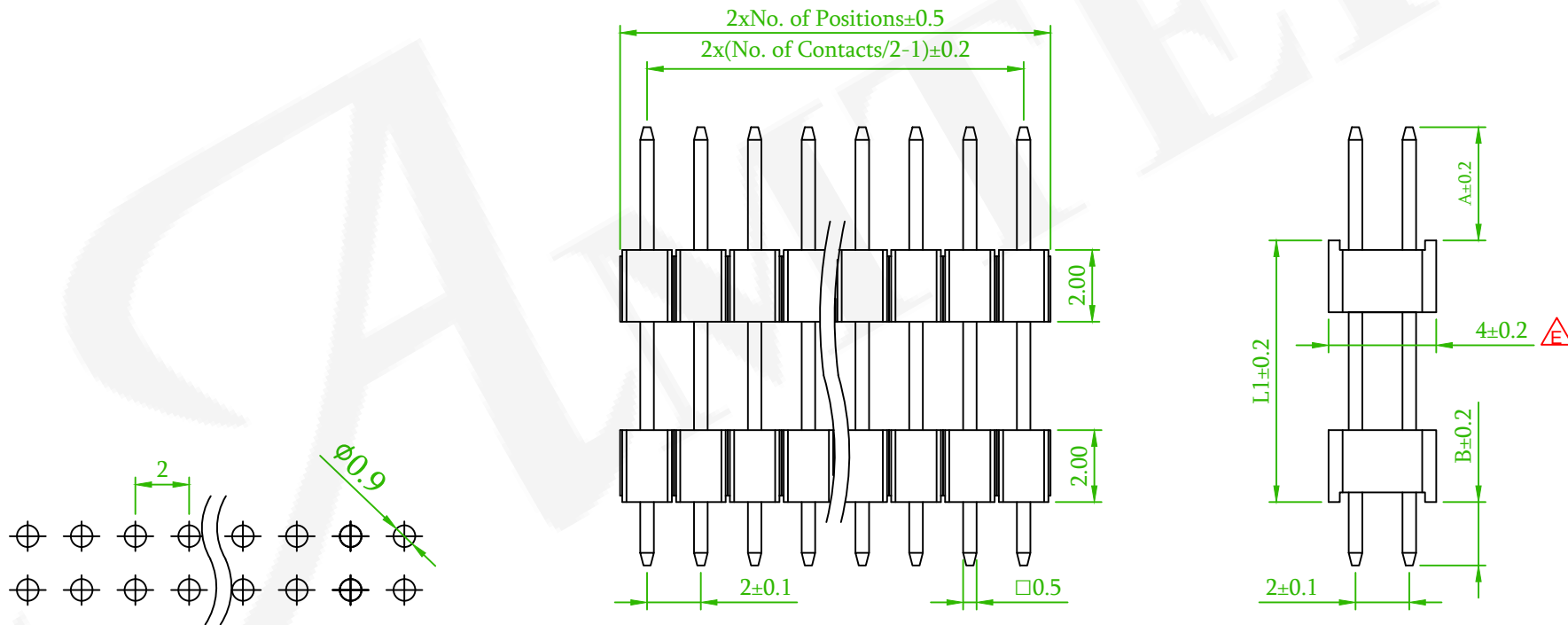
Recommended PCB Layout (PCB TOLERANCE ±0.1)
