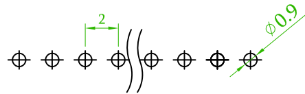
Recommended PCB Layout (PCB TOLERANCE ±0.1)
