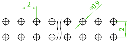
Recommended PCB Layout (PCB TOLERANCE ±0.1)
