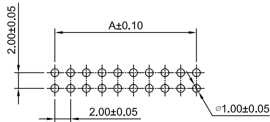
P.C.B LAYOUT (REFERANCE PCB T=1.20~1.60mm)
