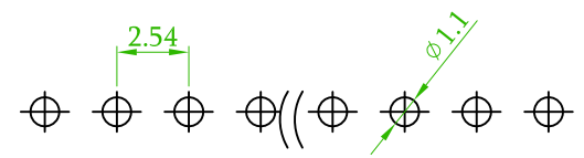
Recommended PCB Layout (PCB TOLERANCE ±0.1)
