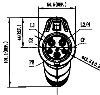
Wiring diagram
