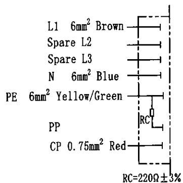
Wiring diagram
