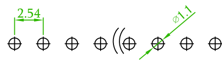
Recommended PCB Layout (PCB TOLERANCE ±0.1)
