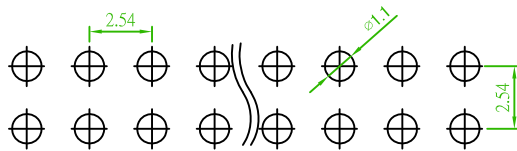
Recommended PCB Layout (PCB TOLERANCE ±0.1)
