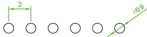
Recommended PCB Layout (PCB TOLERANCE ±0.1)
