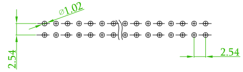
Recommended PCB Layout (PCB TOLERANCE \pm 0.05 , T=1.6/2.0)
