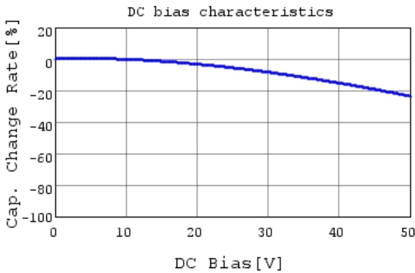
GCM155L81H471KA37 C-DC bias capchange, 25.0c
