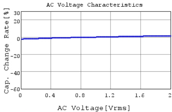
GCM155L81H471KA37 C-AC Voltage capchange, Dc
