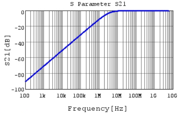
GCM155L81H471KA37 S21 DC0V, 25degC
