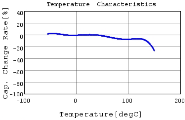
GCM155L81H471KA37 C-Temp. capchange, DC0.0V,
