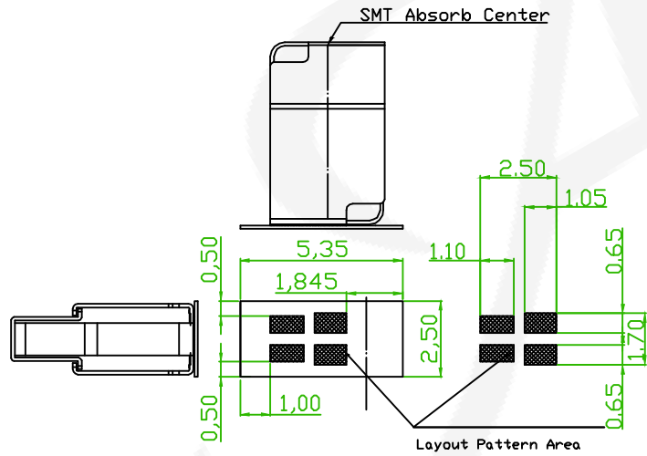
PCB Recommend Layout Pattern
