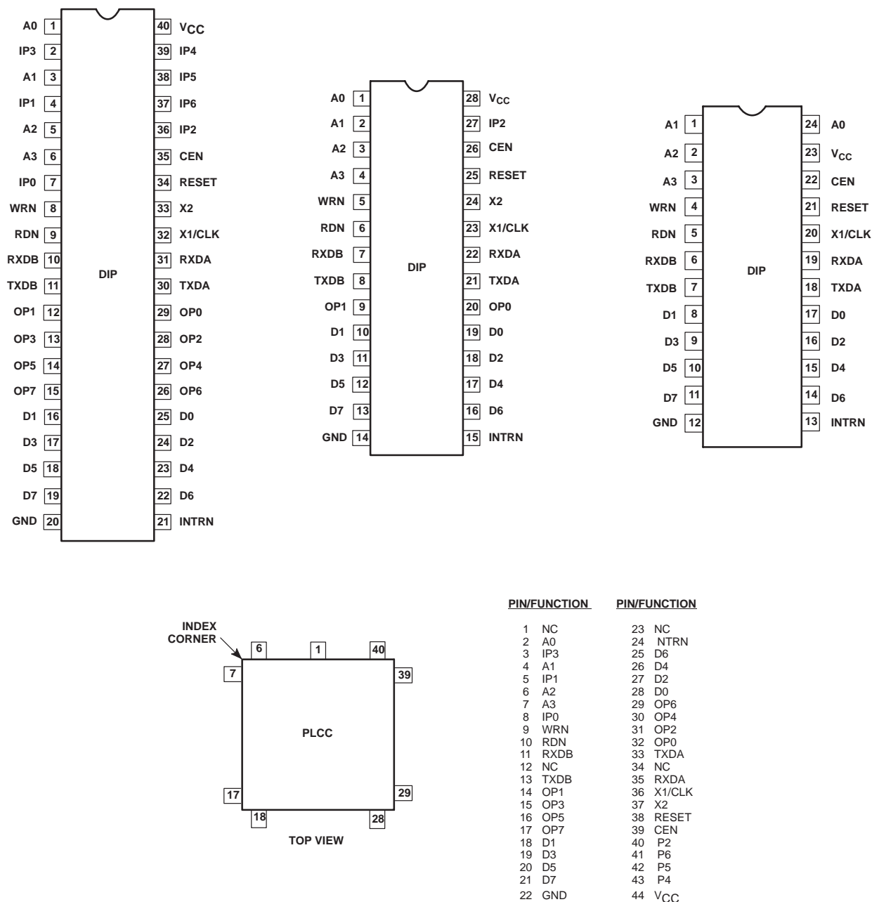
Figure 1. Pin Configurations
