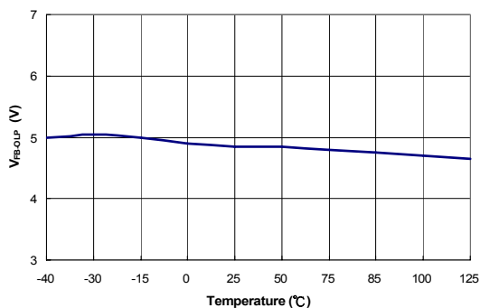
Figure 14. FB Open-Loop Trigger Level ( V_{FB-OLP} ) vs. Temperature
