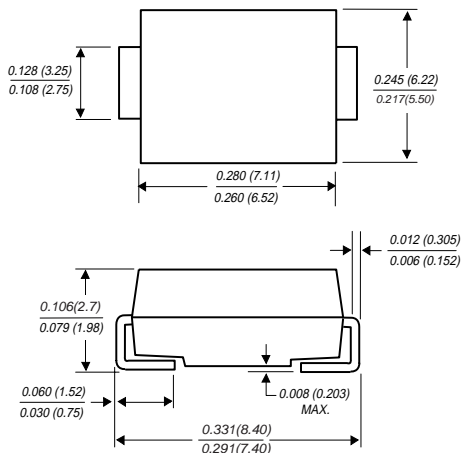
DO-214AB
