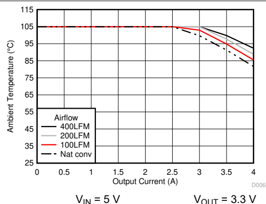
Figure 6-6. Safe Operating Area
