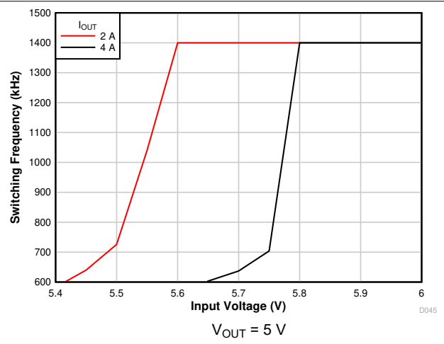
Figure 7-10. Frequency Foldback
