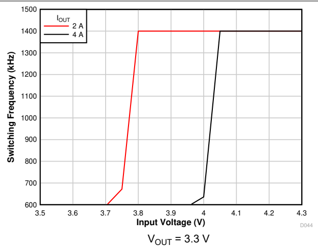
Figure 7-8. Frequency Foldback
