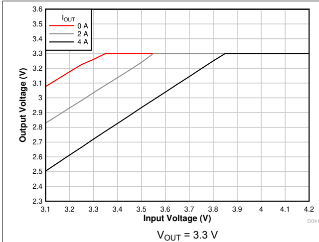
Figure 7-7. Voltage Dropout
