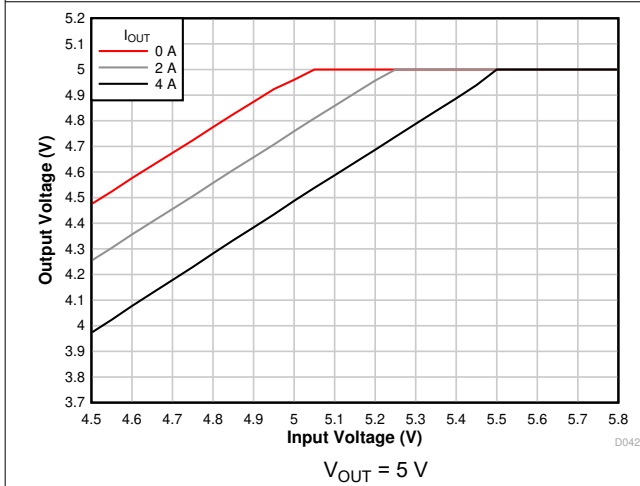
Figure 7-9. Voltage Dropout
