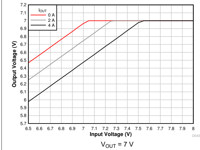
Figure 7-11. Voltage Dropout
