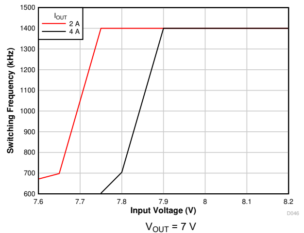
Figure 7-12. Frequency Foldback
