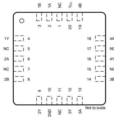
SN54LVC32A FK Package 20-Pin LCCC Top View
