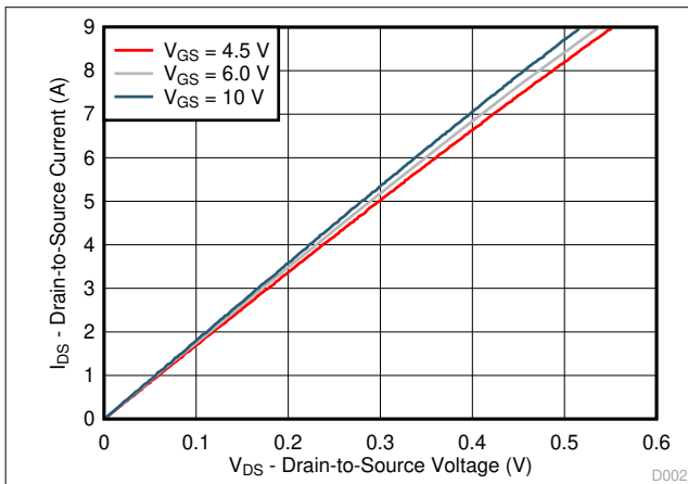
Figure 5-2. Saturation Characteristics
