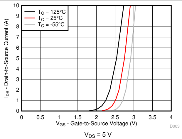
Figure 5-3. Transfer Characteristics
