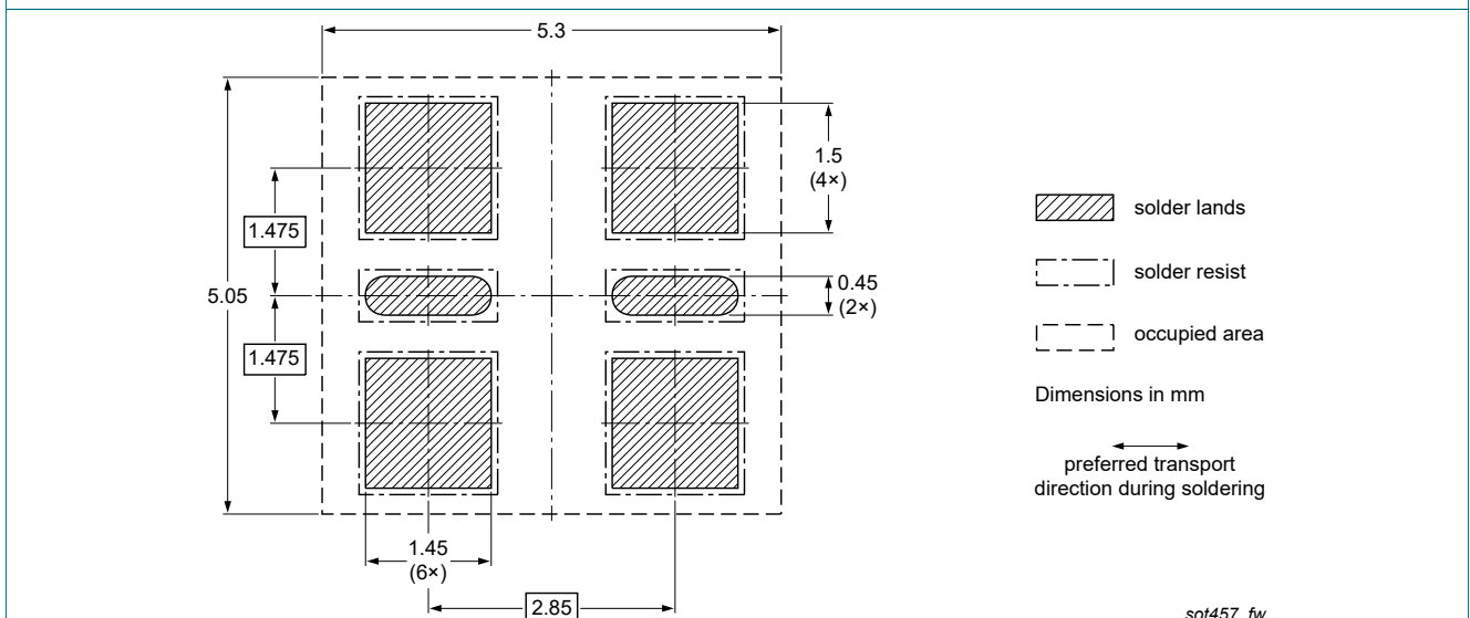
Fig. 7. Wave soldering footprint for TSOP6 (SOT457)
