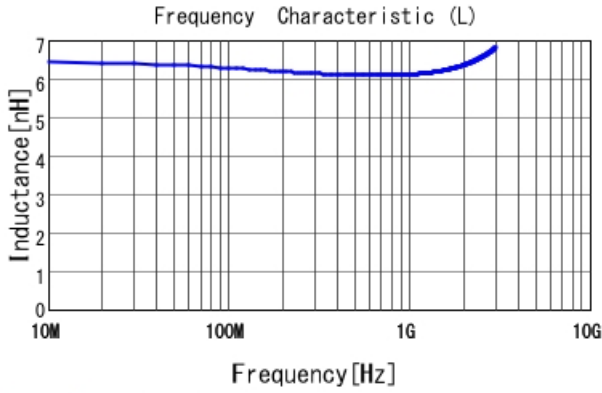
LQW03AW6N2J00 L
