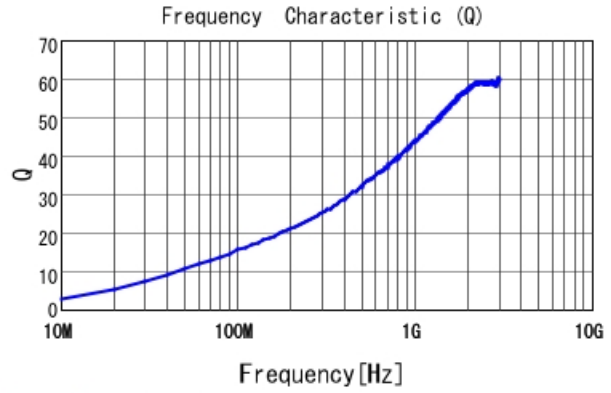
LQW03AW6N2J00 Q
