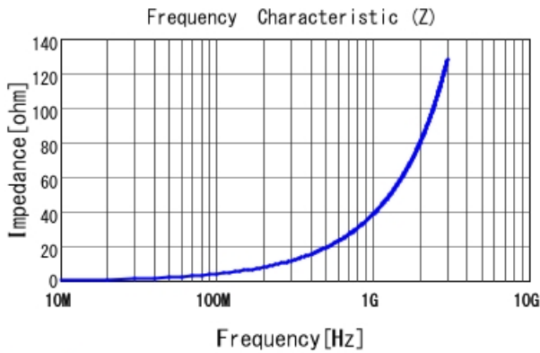
LQW03AW6N2J00 |Z|
