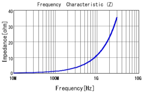
LQP03TN1N8BZ2 |Z|
