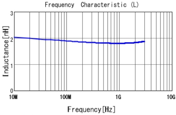
LQP03TN1N8BZ2 L
