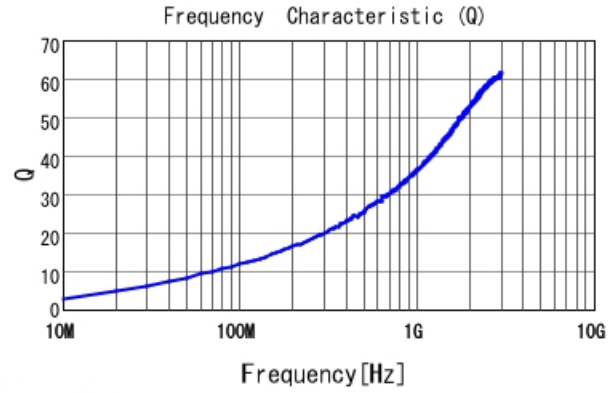
LQP03TN1N8BZ2 Q
