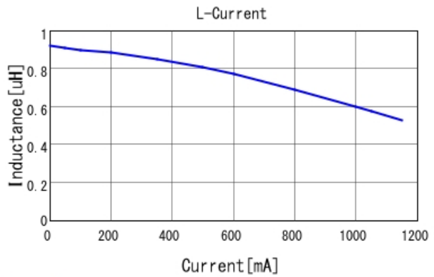
LQM21PN1R0MCH L-Current 20degC
