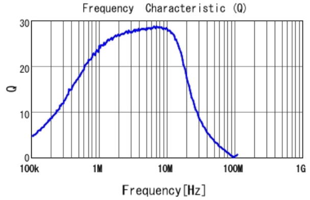
LQM21PN1R0MCH Q
