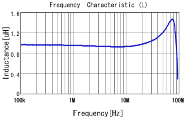
LQM21PN1R0MCH L
