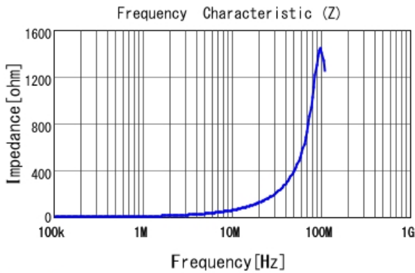
LQM21PN1R0MCH |Z|
