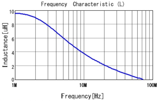
LQM21DN100N00 L
