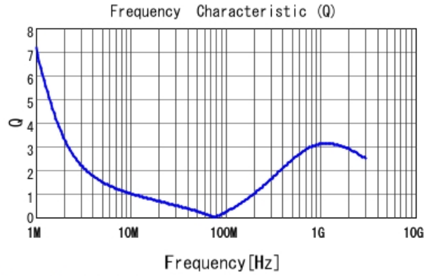
LQM21DN100N00 Q
