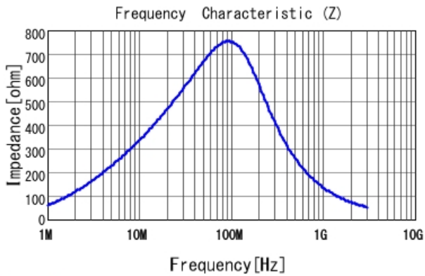
LQM21DN100N00 |Z|
