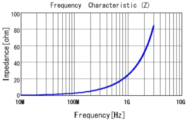
LQG18HN3N9S00 |Z|
