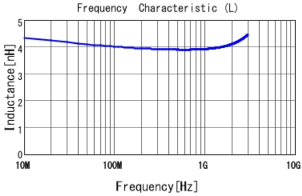
LQG18HN3N9S00 L
