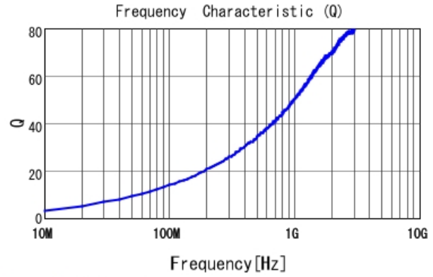
LQG18HN3N9S00 Q
