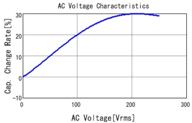
DE2E3SA332MA2BT01F C-AC Voltage capchange, DC0V, 2
