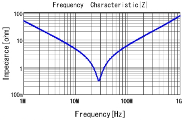
DE2E3SA332MA2BT01F |Z| DC0V, 20degC
