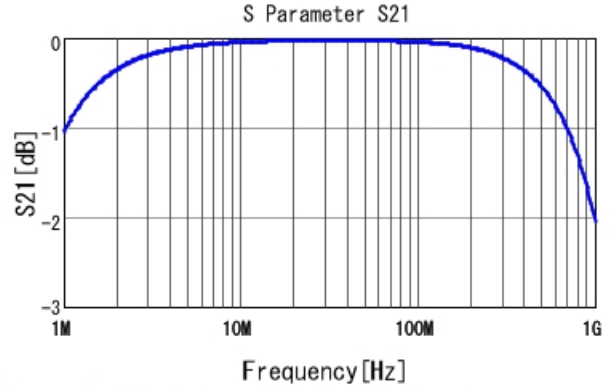
DE2E3SA332MA2BT01F S21 DCOV, 20degC
