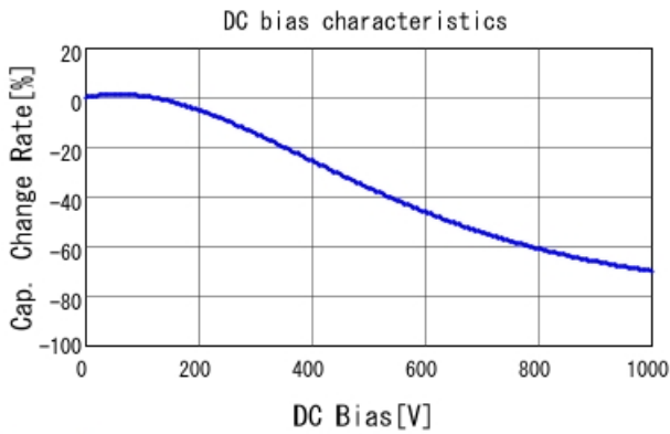
DE2E3SA332MA2BT01F C-DC bias capchange, 20.0degC,
