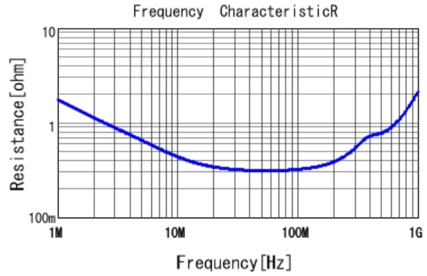
DE2E3SA332MA2BT01F R DC0V, 20degC
