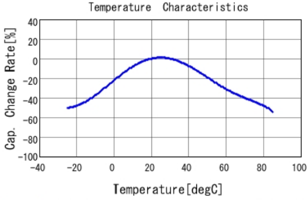
DE2E3SA332MA2BT01F C-Temp. capchange, DCOV, AC1Vrr
