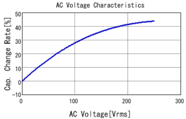
DE2E3KY102MN2AM01F C-AC Voltage capchange, DC0V, 2
