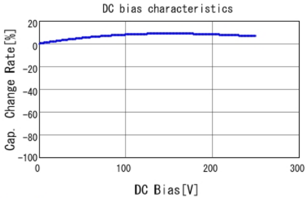
DE2E3KY102MN2AM01F C-DC bias capchange, 20.0degC,
