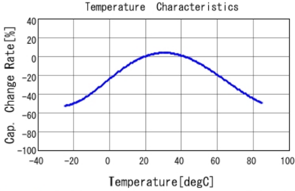
DE2E3KY102MN2AM01F C-Temp. capchange, DCOV, AC1Vrr
