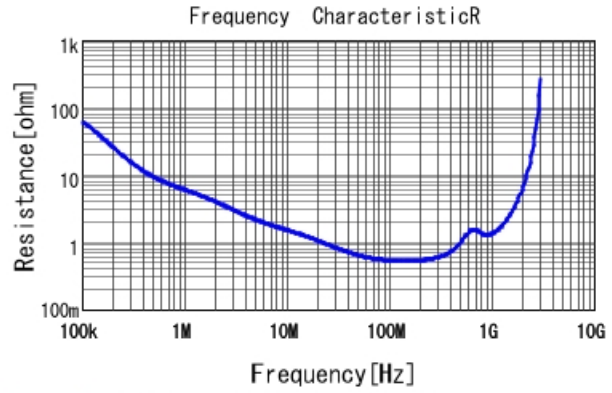
DE2E3KY102MN2AM01F R DC0V, 20degC
