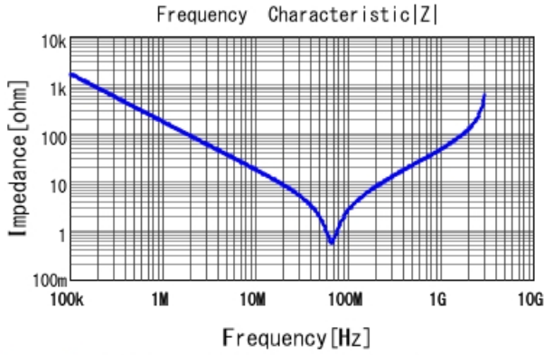
DE2E3KY102MN2AM01F |Z| DC0V, 20degC
