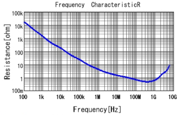
GCM155R71H471KA37 R DCOV, 25degC
