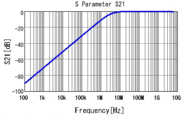
GCM155R71H471KA37 S21 DC0V, 25degC
