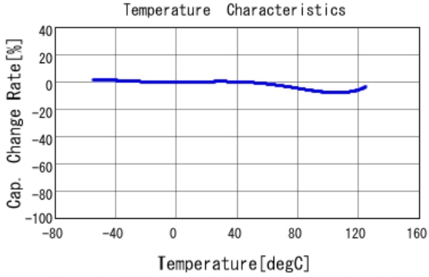
GCM155R71H471KA37 C-Temp. capchange, DC0.0V, AC1.C
