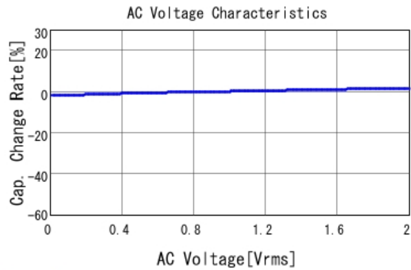
GCM155R71H471KA37 C-AC Voltage capchange, DCOV, 25
