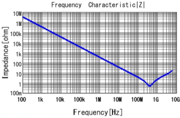
GCM155R71H471KA37 |Z| DCOV, 25degC
