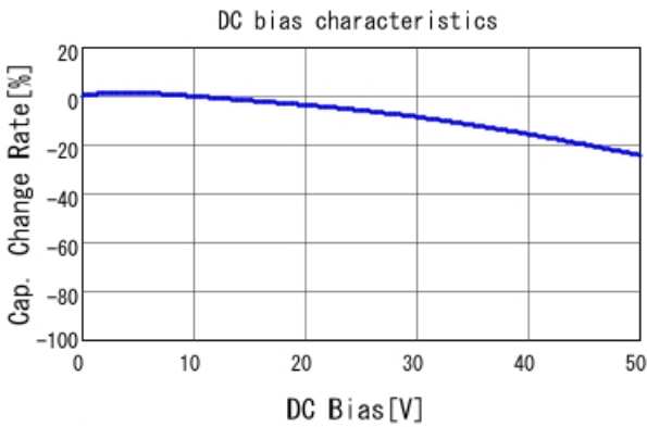
GCM155R71H471KA37 C-DC bias capchange, 25.0degC, A
