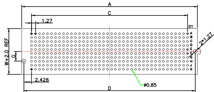
Recommended PCB Layout (BGA)
