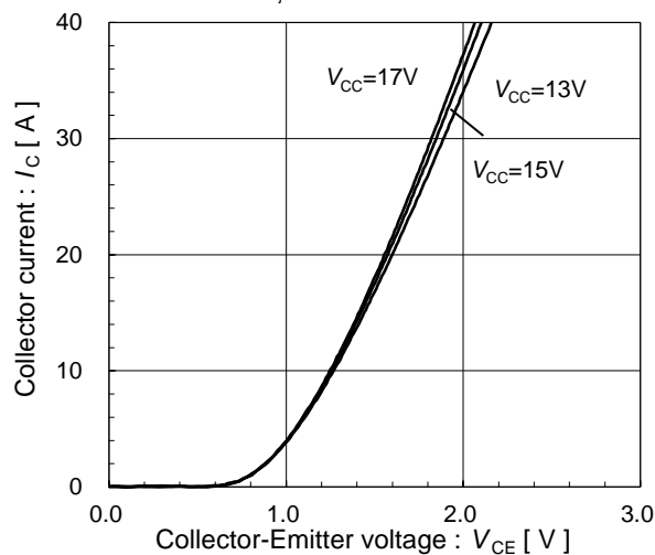
Collector current vs. Collector-Emittor voltage (typ.) T_{vj}=25^{\circ}\text{C} [ Terminal ]
