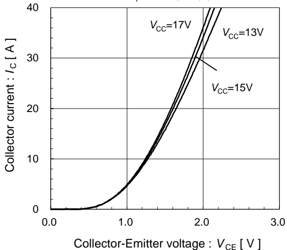
Collector current vs. Collector-Emittor voltage (typ.) T_{vj}=125^{\circ}\text{C} [ Chip ]
