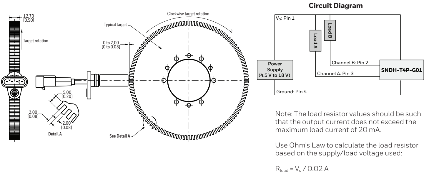
FIGURE 5. SNDH-T4P-G01 DIMENSIONAL DRAWINGS (FOR REFERENCE ONLY: MM [IN].)
