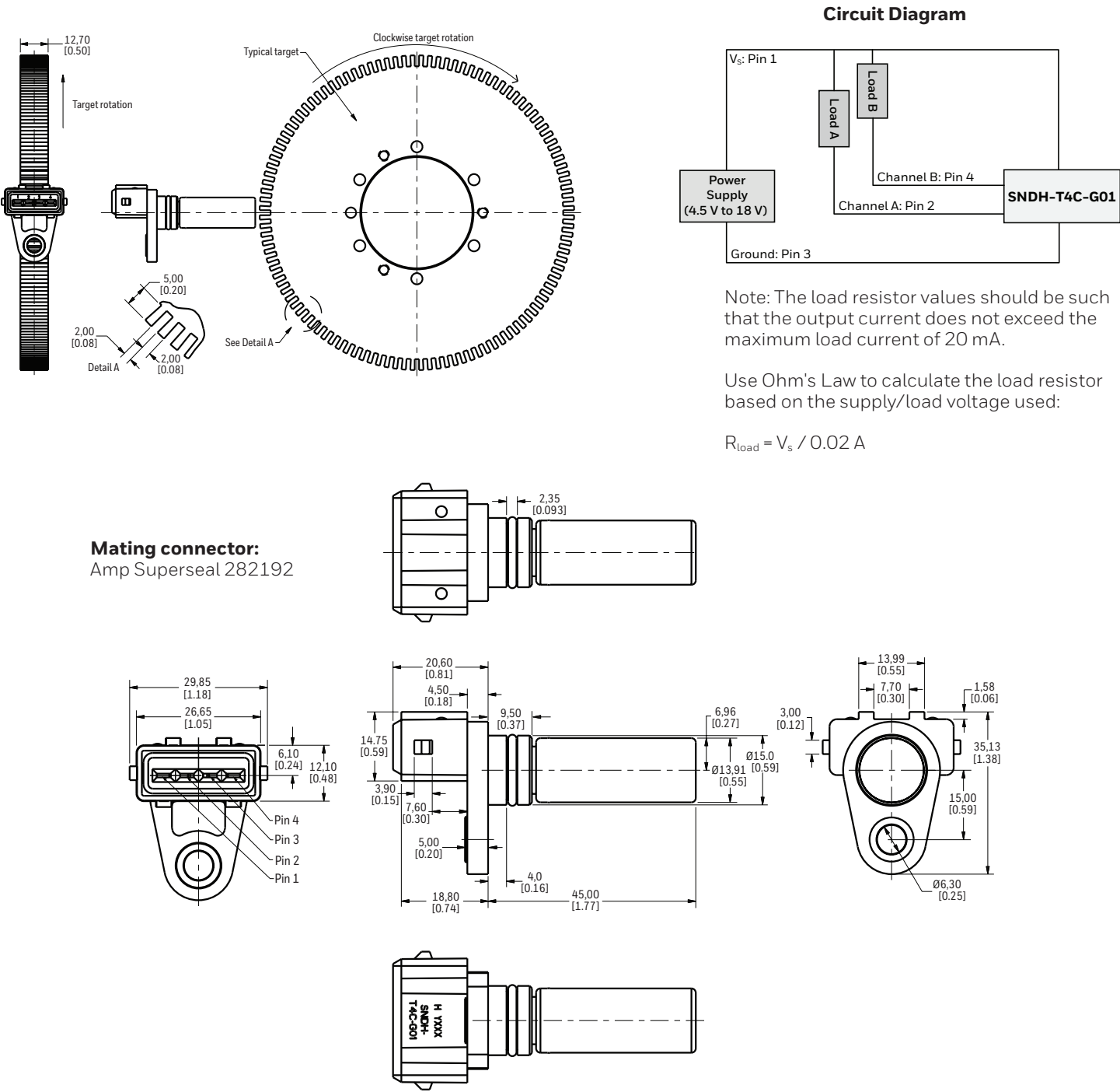
FIGURE 3. SNDH-T4C-G01 DIMENSIONAL DRAWINGS (FOR REFERENCE ONLY: MM [IN]).
