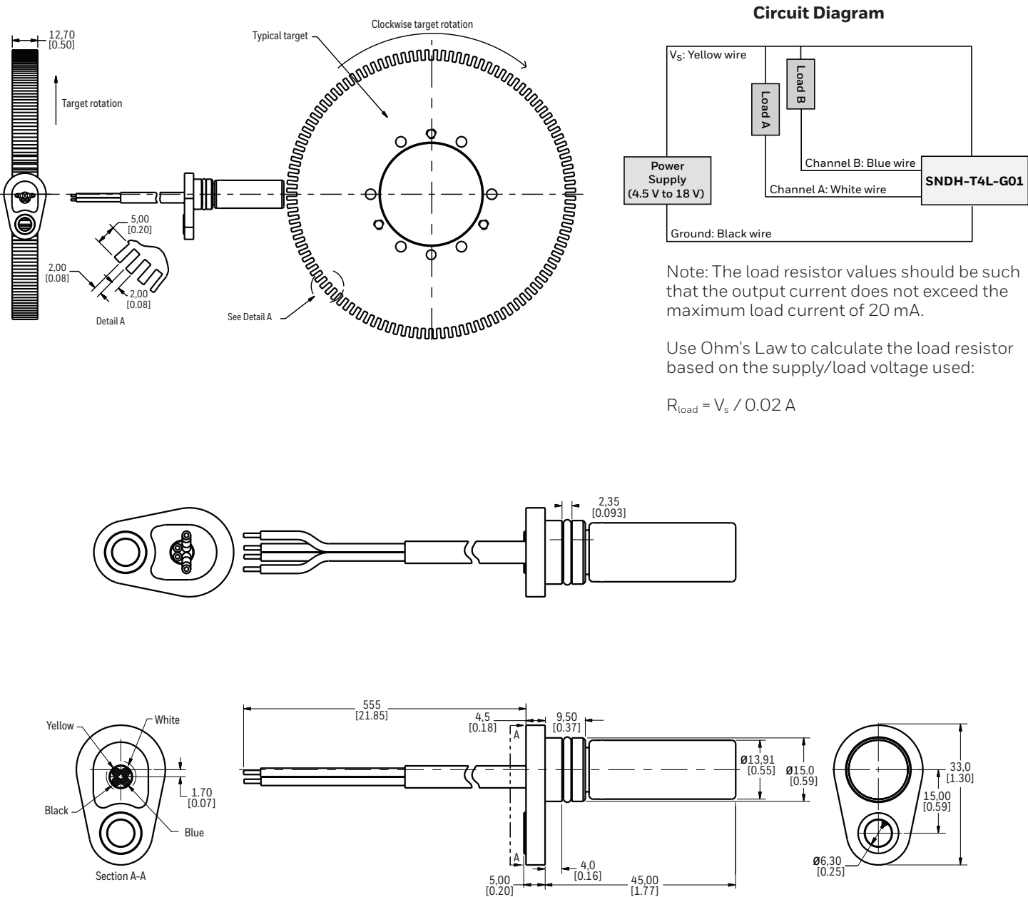
FIGURE 4. SNDH-T4L-G01 DIMENSIONAL DRAWINGS (FOR REFERENCE ONLY: MM [IN.])
