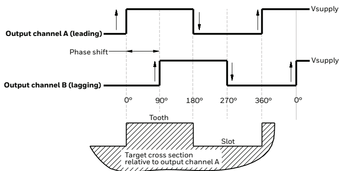
FIGURE 1. SENSOR OUTPUT
