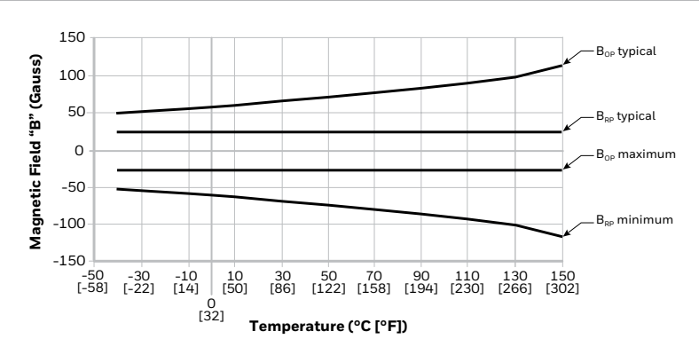
Figure 1. Magnetic Characteristics vs Temperature
