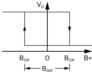
Figure 3. Transfer Characteristics
