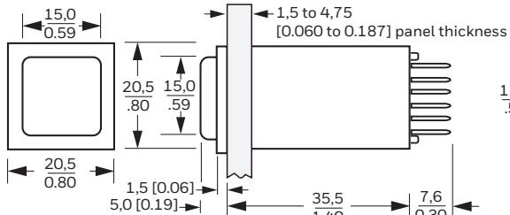
AML21 Series Square
