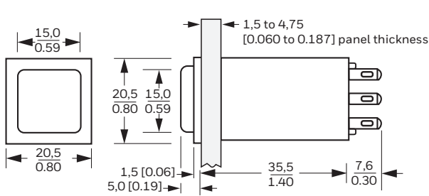
AML21 Series Square
