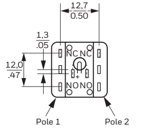
0.020 in x 0.110 in Termination
