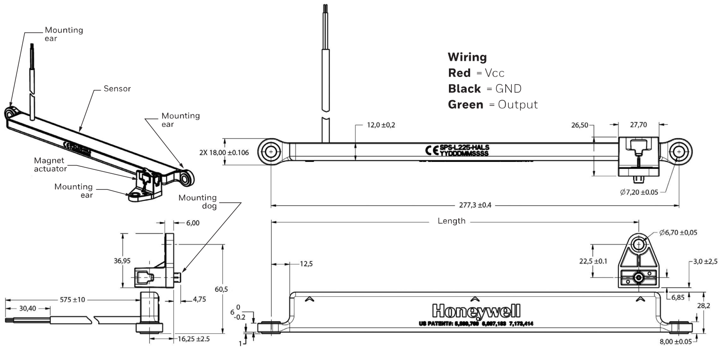
FIGURE 3. SPS-L225-HALS MOUNTING DIMENSIONS (FOR REFERENCE ONLY: MM) AND SENSOR OUTPUT PERFORMANCE GRAPH
