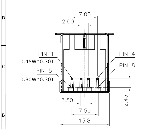
RECOMMEND LAYOUT (TOP VIEW) GENERAL TOLERANCE: \pm 0.1\text{mm}
