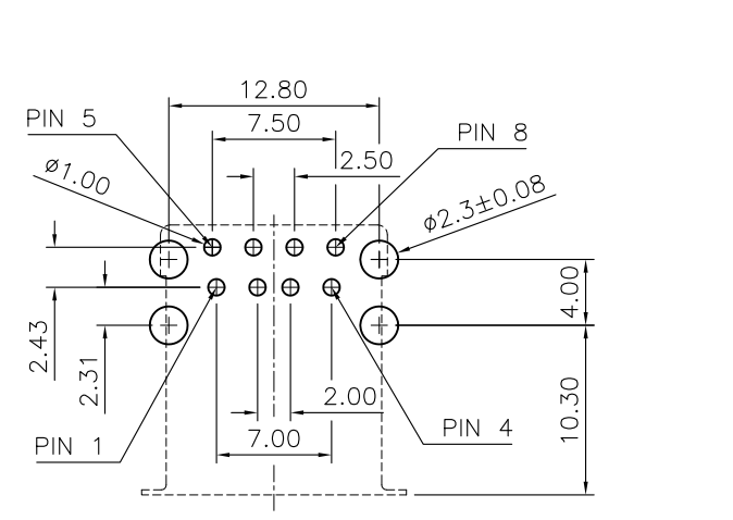
RECOMMEND LAYOUT (TOP VIEW) GENERAL TOLERANCE: \pm 0.1\text{mm}
