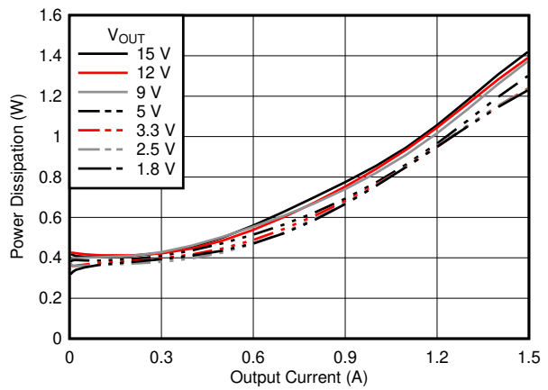
Figure 7-8. Power Dissipation
