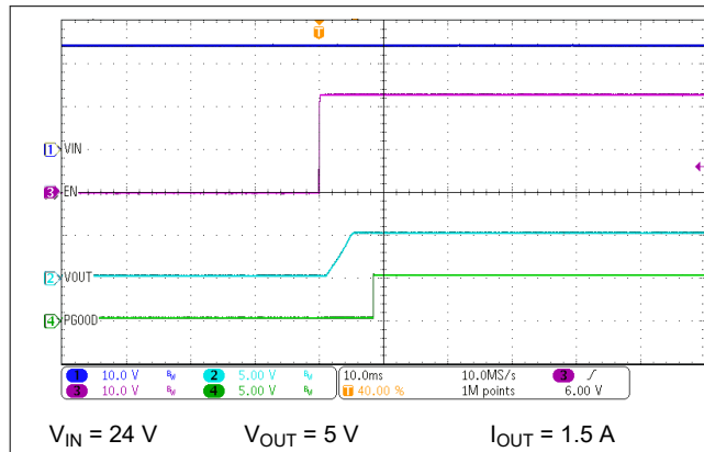
Figure 9-2. Start-up Waveforms
