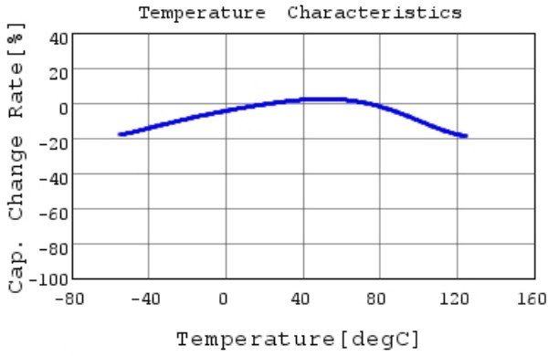
GRT21BC71H475KE13 C-Temp. capchange, DC0.0V,
