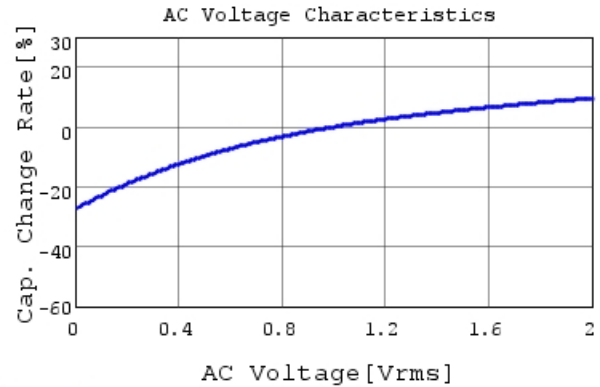
GRT21BC71H475KE13 C-AC Voltage capchange, Dc
