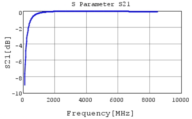
GJM0335C1E6R0CB01 S21 DCOV, 25degC
