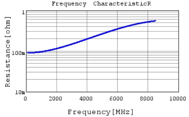
GJM0335C1E6R0CB01 R DCOV, 25degC
