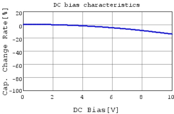
GRM31MR71A225KA01 C-DC bias capchange, 25.0c
