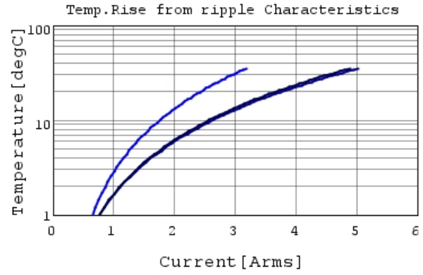
GRM31MR71A225KA01 Temp.rise — 100kHz —
