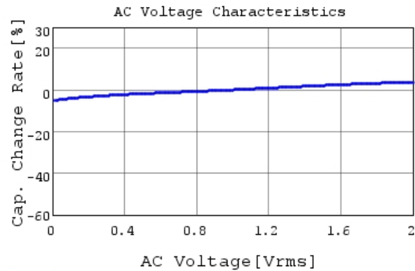
GRM31MR71A225KA01 C-AC Voltage capchange, Dc
