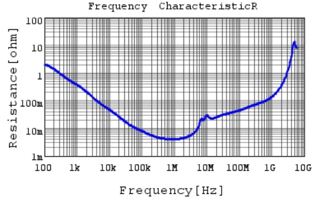
GRM31MR71A225KA01 R DCOV, 25degC
