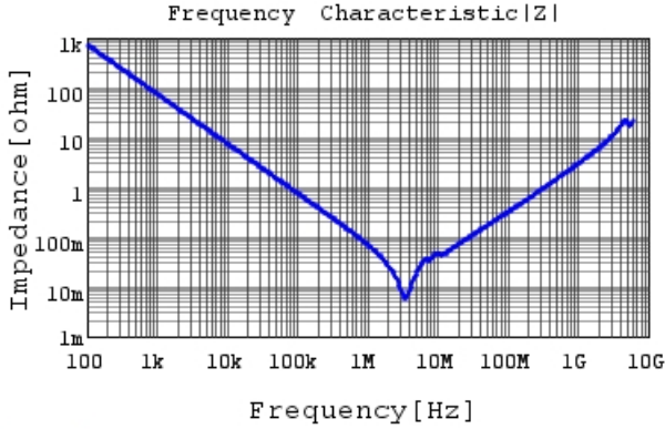
GRM31MR71A225KA01 |Z| DCOV, 25degC
