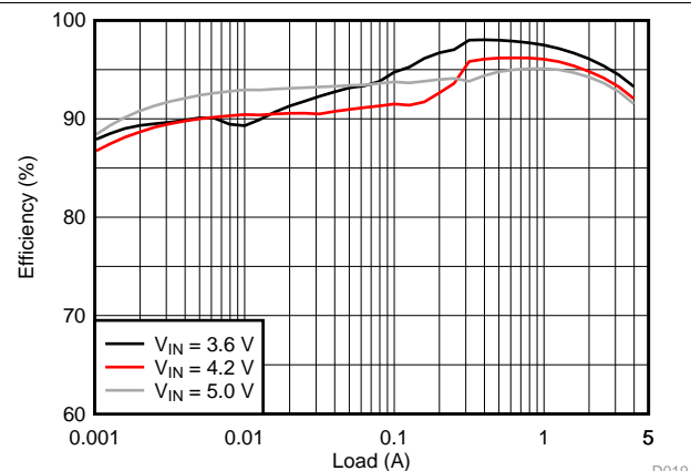
Figure 25. 3.3V Output Application Efficiency
