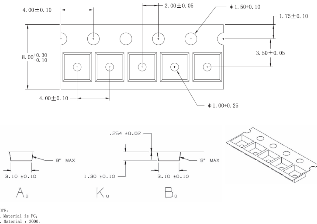
Figure 9.6: TSOT23-6 Tape Specification.
