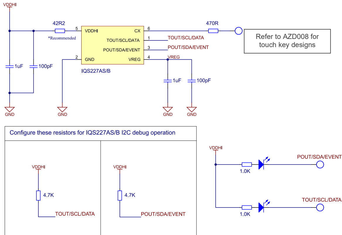
Figure 2.3: Typical application schematic of IQS227AS/B. 100pF capacitors are optional for added RF immunity. Place all decoupling capacitors (on VDDHI and VREG) as close to the IC as possible.
