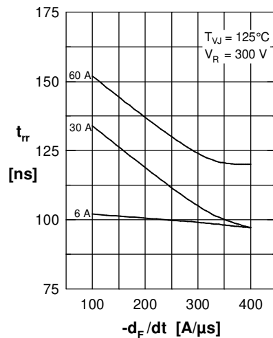
Fig. 5 Typ. recovery time t_{rr} versus -d_F/dt
