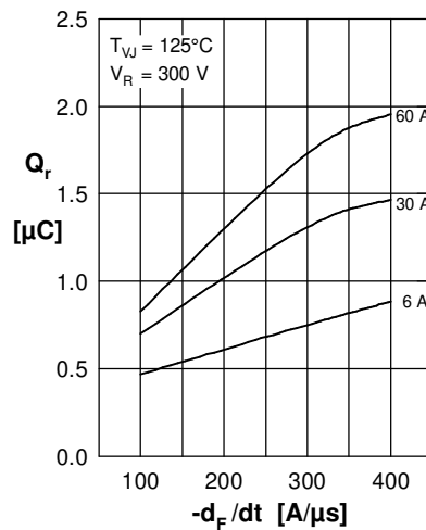
Fig. 2 Typ. reverse recov. charge Q_r versus -d_F/dt
