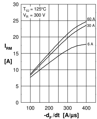
Fig. 3 Typ. peak reverse current I_{RM} versus -d_F/dt
