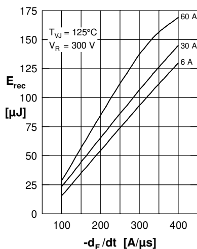
Fig. 7 Recovery energy versus -d_F/dt
